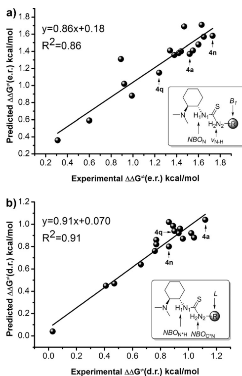
Figure 3. FER analysis for all catalysts.
