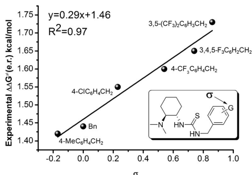
Figure 2. FER analysis of the electronic effects of benzyl-substituted thioureas.
