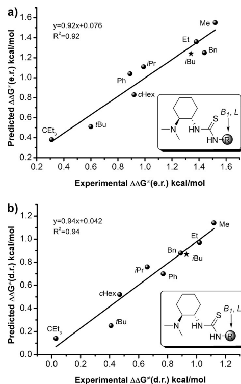
Figure 1. FER analysis of steric effects.
