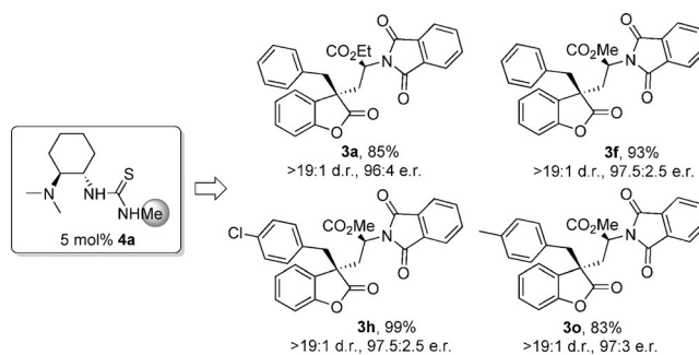
Scheme 2. Catalytic performance of methyl catalyst 4a . Reaction conditions: 1 (0.1 mmol), 2 (0.15 mmol), 4a (5 mol %), 3 Å molecular sieves (40 mg), chlorobenzene (1.0 mL), -30^\circ\text{C} , 5 days.
